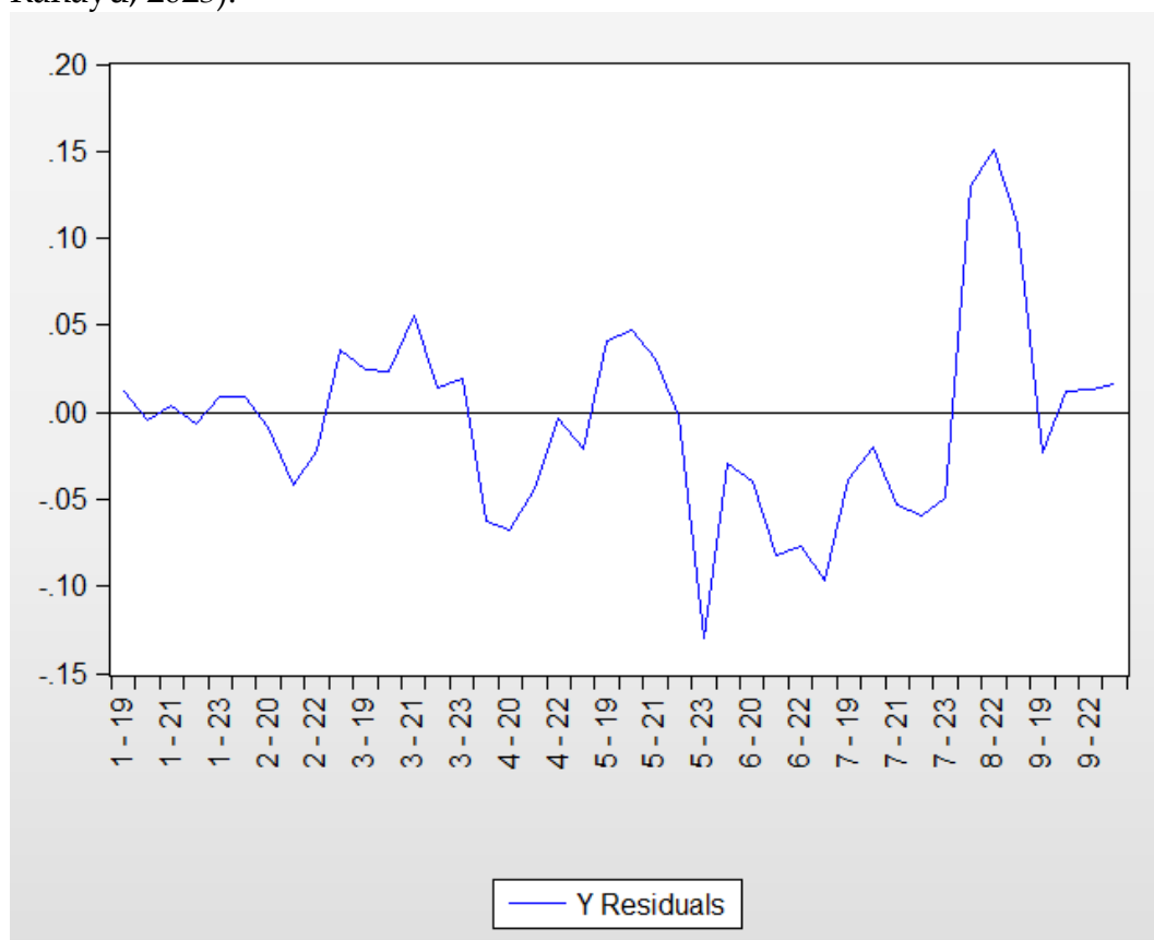
Figure 2. Heteroscedasticity Test Results
